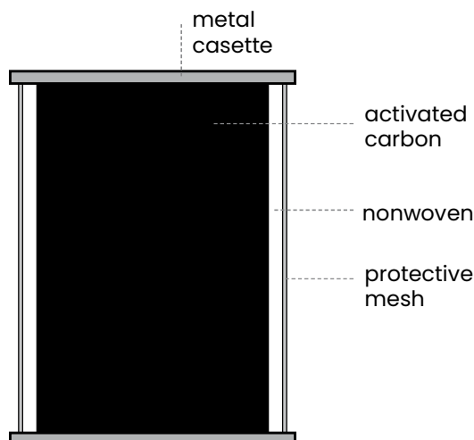
UltraSorb KP filter cross-section
