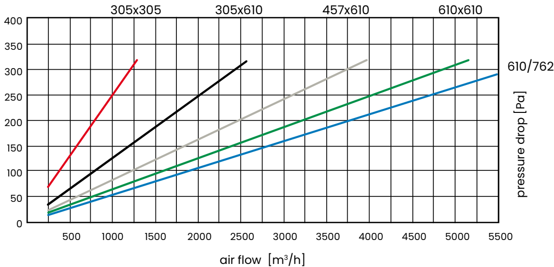
Pressure drop diagram for H13 class filters with an enlarged filtration area
