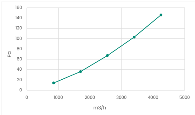
592x592x96 [mm]
