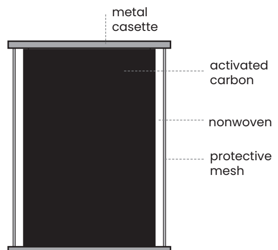
UltraSorb KP filter cross-section
